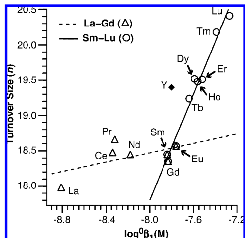
Figure 5. Turnover size plotted versus the first hydrolysis constant, \log^0 \beta_1(M) , 57 for each trivalent metal ion studied in bulk aqueous solutions. Linear best fits are shown for La–Gd (dashed line) and Sm–Lu (solid line). Note that the elements near the middle of the lanthanide series, Sm, Eu, and Gd, are included with both sets.
